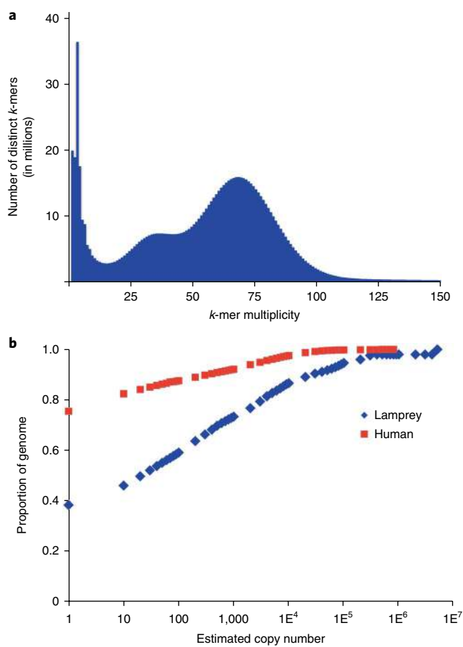
Fig. 1 | Distribution of k -mer copy numbers in germline shotgun
