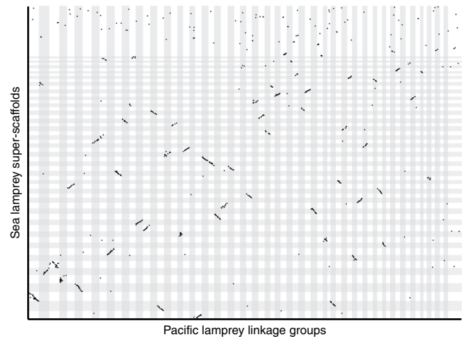
Fig. 3 | Alignment of the Pacific lamprey ( E. tridentatus ) meiotic map to assembled sea lamprey ( P. marinus ) super-scaffolds. The relative position of homologous sequences is shown for sea lamprey (y axis) and Pacific lamprey (x axis). A single homologous site (aligning RAD-seq read, Supplementary Table 1) is marked by a single dot. Chromosomes and linkage groups (LGs) are ordered from longest to shortest within species, and individual chromosomes and LGs are highlighted by alternating dark and light shading. Groups of adjacent dots (regions showing conservation of synteny and gene order) appear as diagonal lines.
