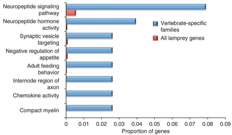
Figure 5. Enrichment of gene ontologies among vertebrate-specific gene families. Horizontal bars show the frequencies of ontology classes among vertebrate-specific gene families and in the entire set of lamprey gene models. Data are shown for all ontologies that are over-represented with P < 0.005 (Fisher's exact test). Most over-represented ontologies are related to neural development and neurohormone signaling.
