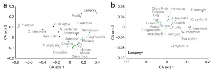
Figure 2. Genome-wide deviation of lamprey coding sequence properties from patterns observed in other vertebrate and invertebrate genomes. (a) Codon usage bias. Correspondence analysis (CA) on relative synonymous codon usage (RSCU) values was performed using the nucleotide sequences of all predicted genes concatenated for individual species. (b) Amino-acid composition. Red, lamprey; gray, invertebrates; green, jawed vertebrates.
