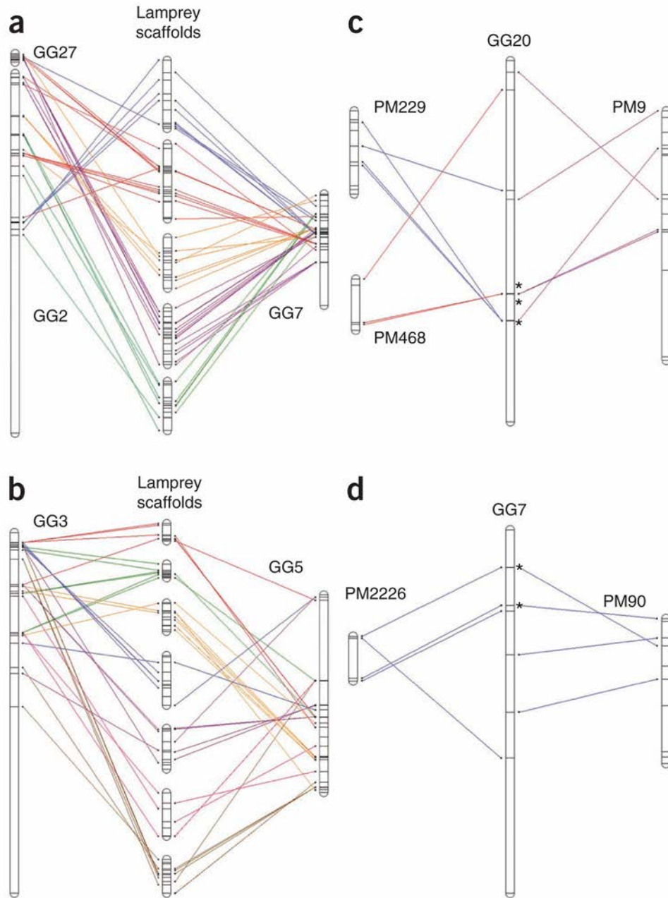
Figure 3. Conserved synteny and duplication in the lamprey and gnatostome (chicken) genomes. (a–d) The locations of presumptive lamprey-chicken orthologs (including duplicates) are plotted relative to their physical positions on chromosomes and scaffolds and are connected by colored lines. (a,b) Pairs of chicken chromosomes that correspond to a series of lamprey scaffolds. (a) Ten lamprey loci are present as duplicate copies in the chicken genome, and 59 are present as single copies. (b) Twelve lamprey loci are present as duplicate copies in the chicken genome, and 54 are present as single copies. (c,d) Pairs of lamprey scaffolds that correspond to individual chicken chromosomes. (c) Three chicken loci are present as duplicate copies on syntenic lamprey scaffolds. (d) Two chicken loci are present as duplicate copies on syntenic lamprey scaffolds. Asterisks indicate duplicates.
