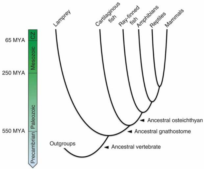
Figure 1. An abridged phylogeny of the vertebrates. Shown is the timing of major radiation events within the vertebrate lineage. Extinct lineages and some extant lineages (for example, coelacanths, lungfish and hagfish) have been omitted for simplicity. Here, reptile is synonymous with sauropsid, ray-finned fish is synonymous with actinopterygian, and osteichthyan is synonymous with euteleostome. CZ, Cenozoic; MYA, million years ago.
